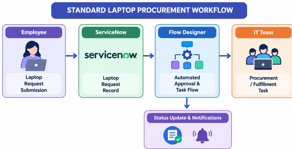
Figure 1: Architecture and workflow of the Standard Laptop Procurement Automation process
